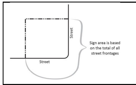
Figure 20.[184]-A—Sign Area Frontage
