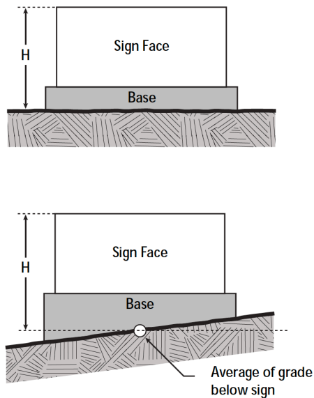
Figure 20.184-C—Measuring Sign Height
