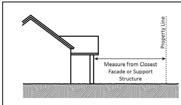
Figure 20.152-C—Measuring Distances from Support Structures
