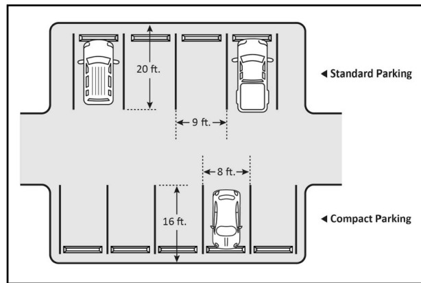
Figure 20.180-A—Parking Space Dimensions
