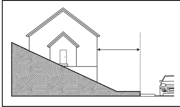
Figure 20.152-B—Measuring Setbacks Along Slopes
