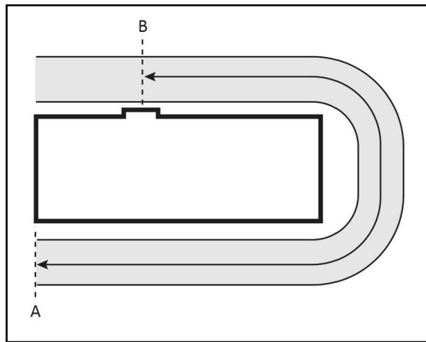
Figure 20.152-D—Measuring Vehicle Stacking and Travel Areas
