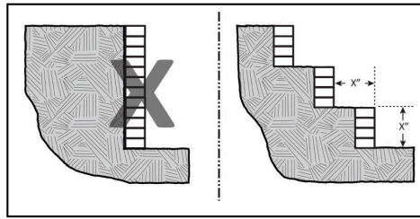
Figure 20.152-P—Retaining Wall Step Design Illustration
